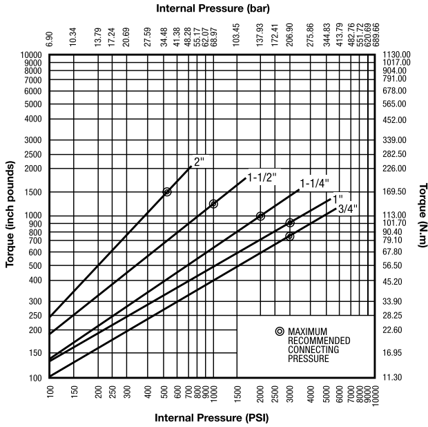
Torque Values for Connecting Under Pressure
